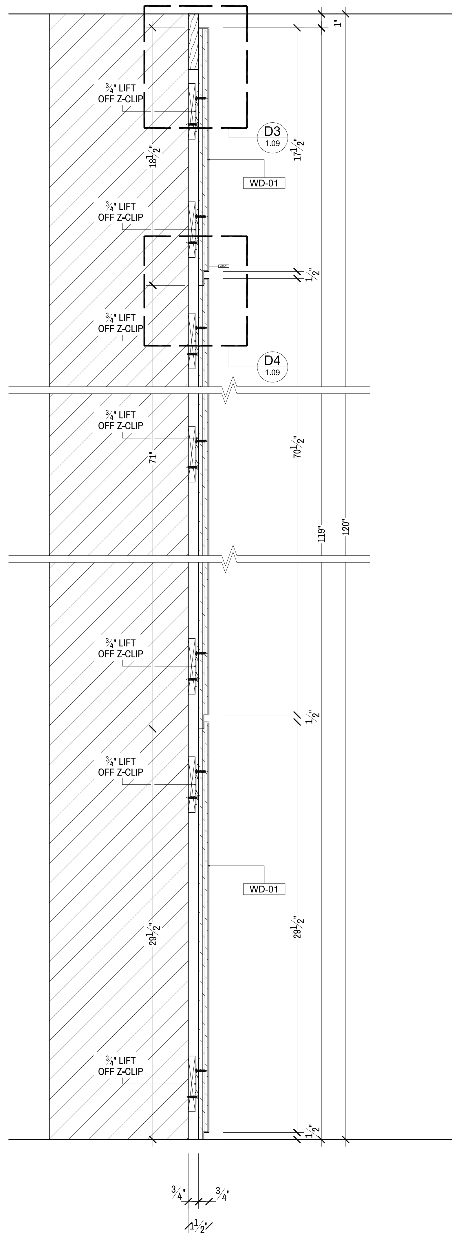
S7 SECTION SCALE: 3/8"=1'-0" RECEPTION RECEPTION 105
