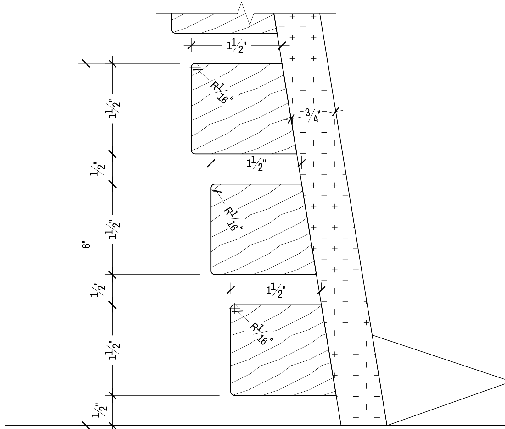
D1 DETAIL SCALE: FULL RECEPTION RECEPTION 105
