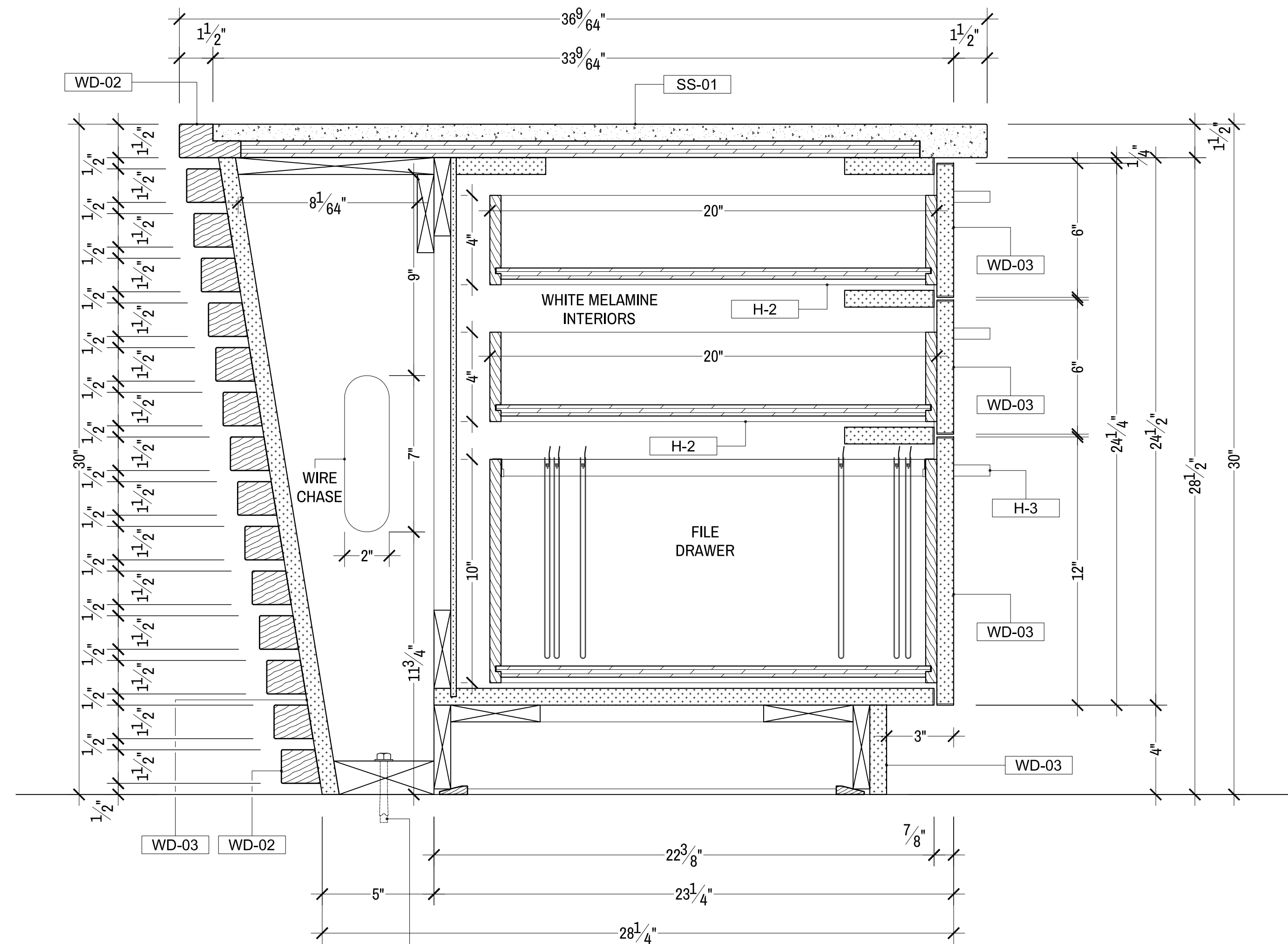
S6 SECTION SCALE: 3"=1'-0" RECEPTION RECEPTION 105
