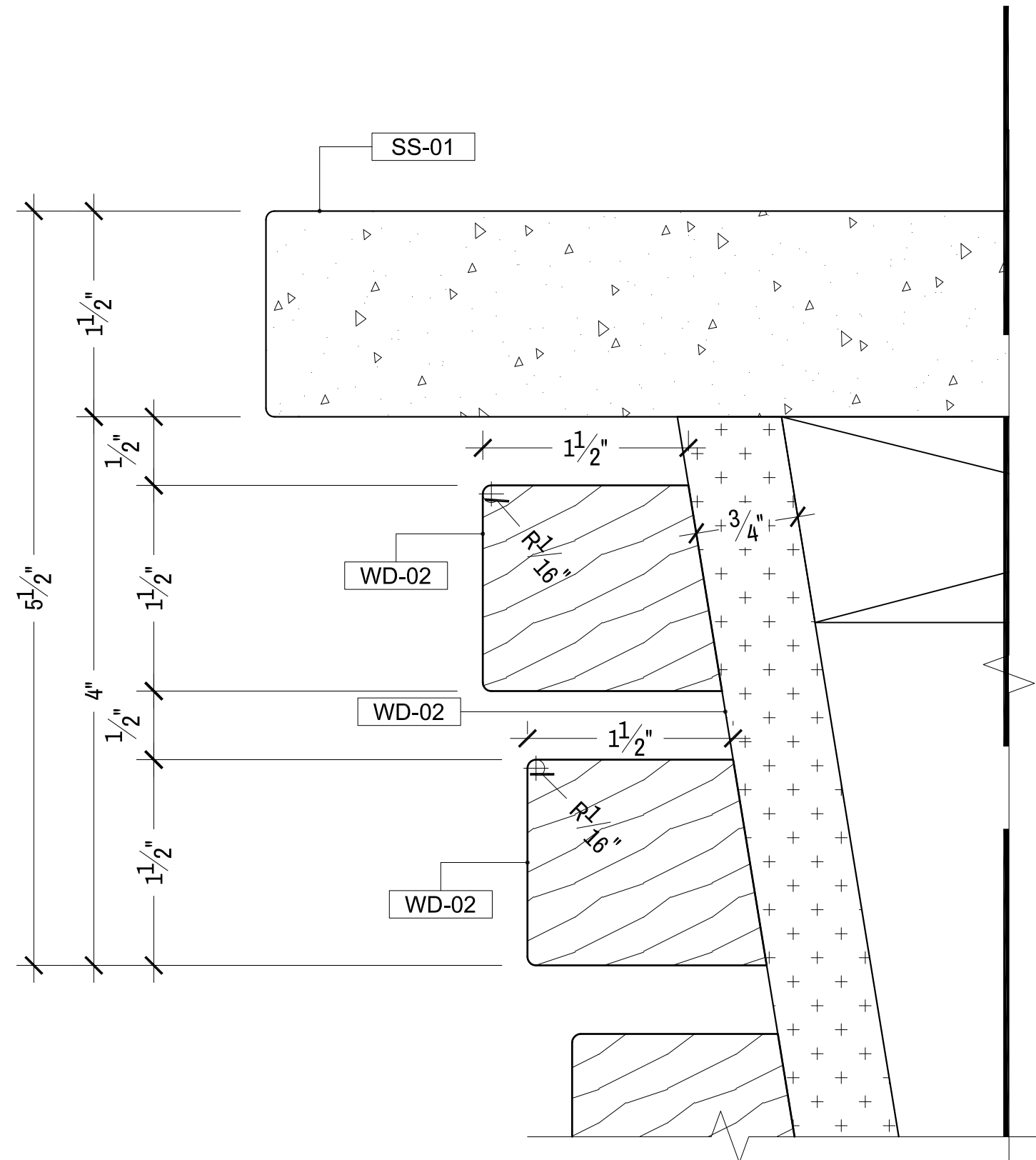
D1 DETAIL SCALE: FULL RECEPTION RECEPTION 105
