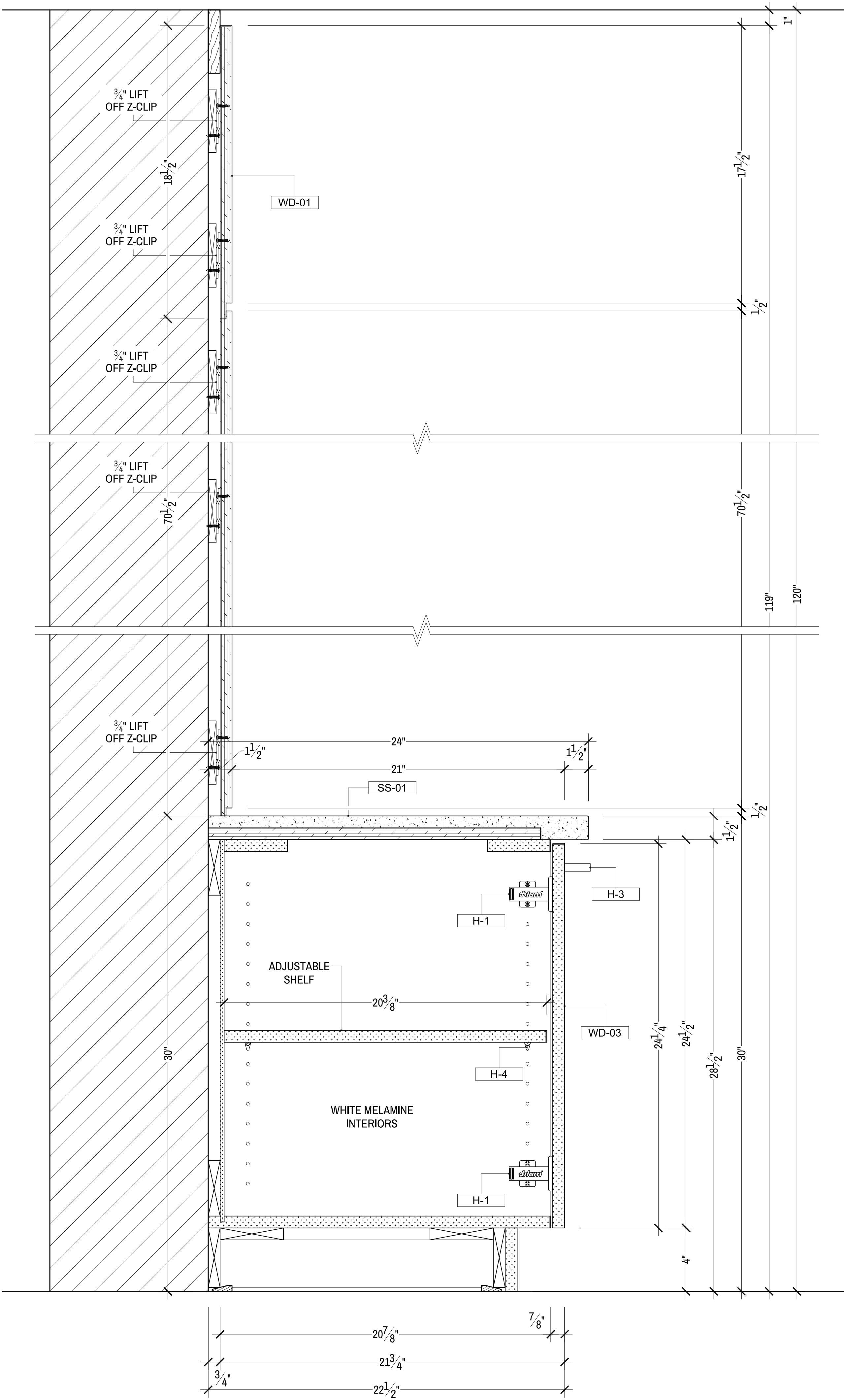
S1 SECTION SCALE: 3"=1'-0" RECEPTION RECEPTION 105
