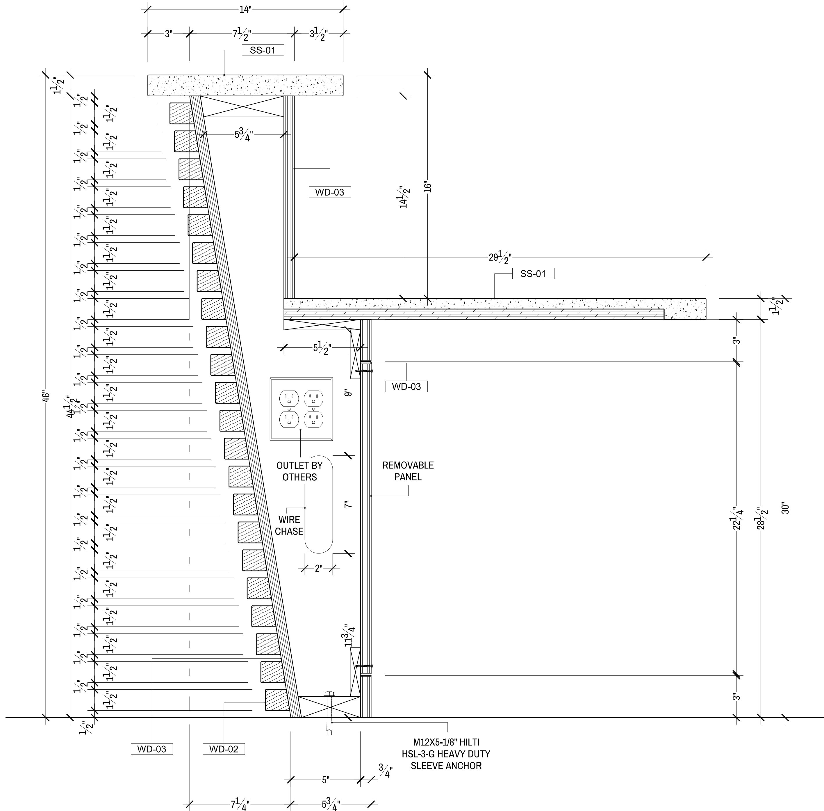
S5 SECTION SCALE: 3"=1'-0" RECEPTION RECEPTION 105
