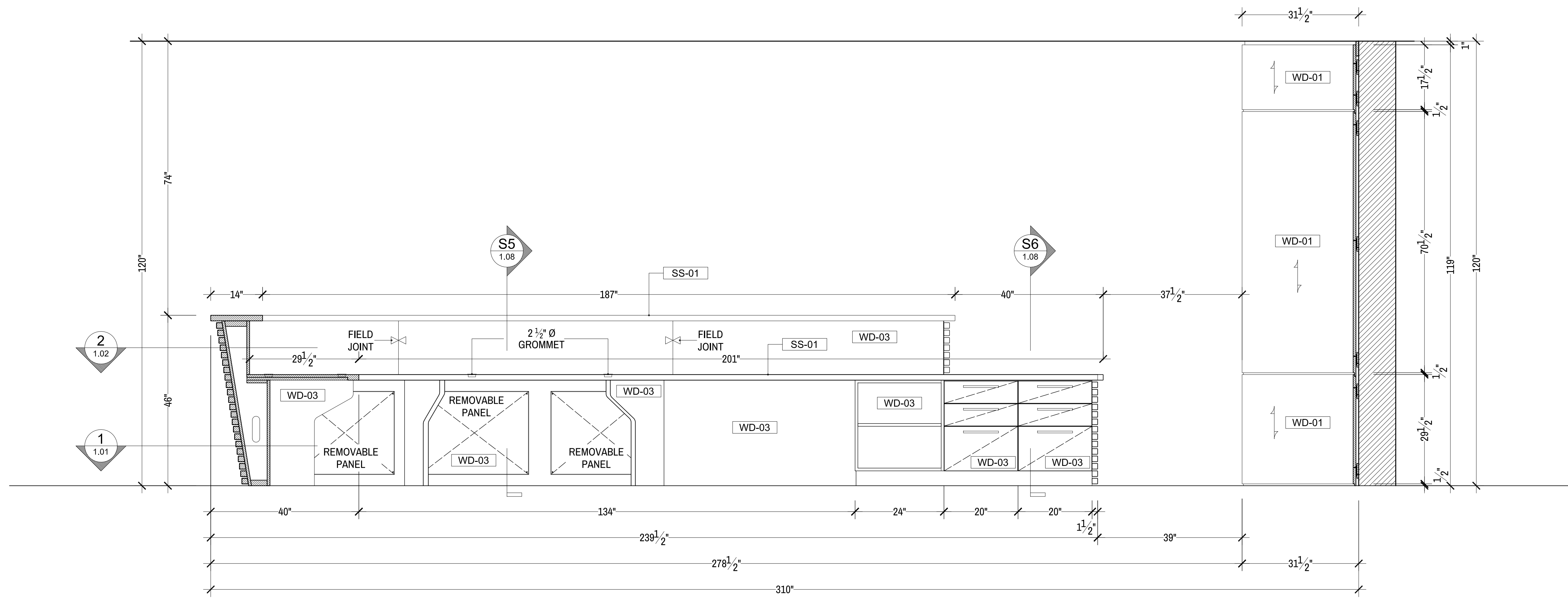
C ELEVATION RECEPTION SCALE: 3/4"=1'-0" RECEPTION 105
