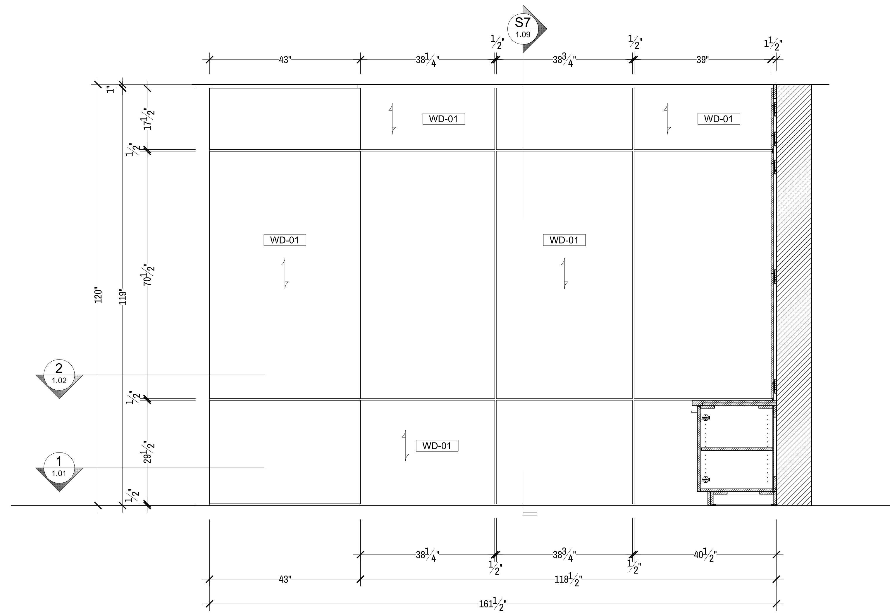
D ELEVATION RECEPTION SCALE: 3/4"=1'-0" RECEPTION 105
