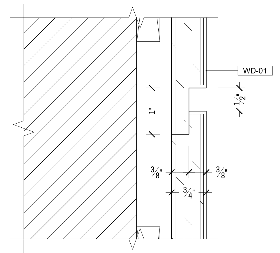
D4 DETAIL SCALE: FULL RECEPTION RECEPTION 105
