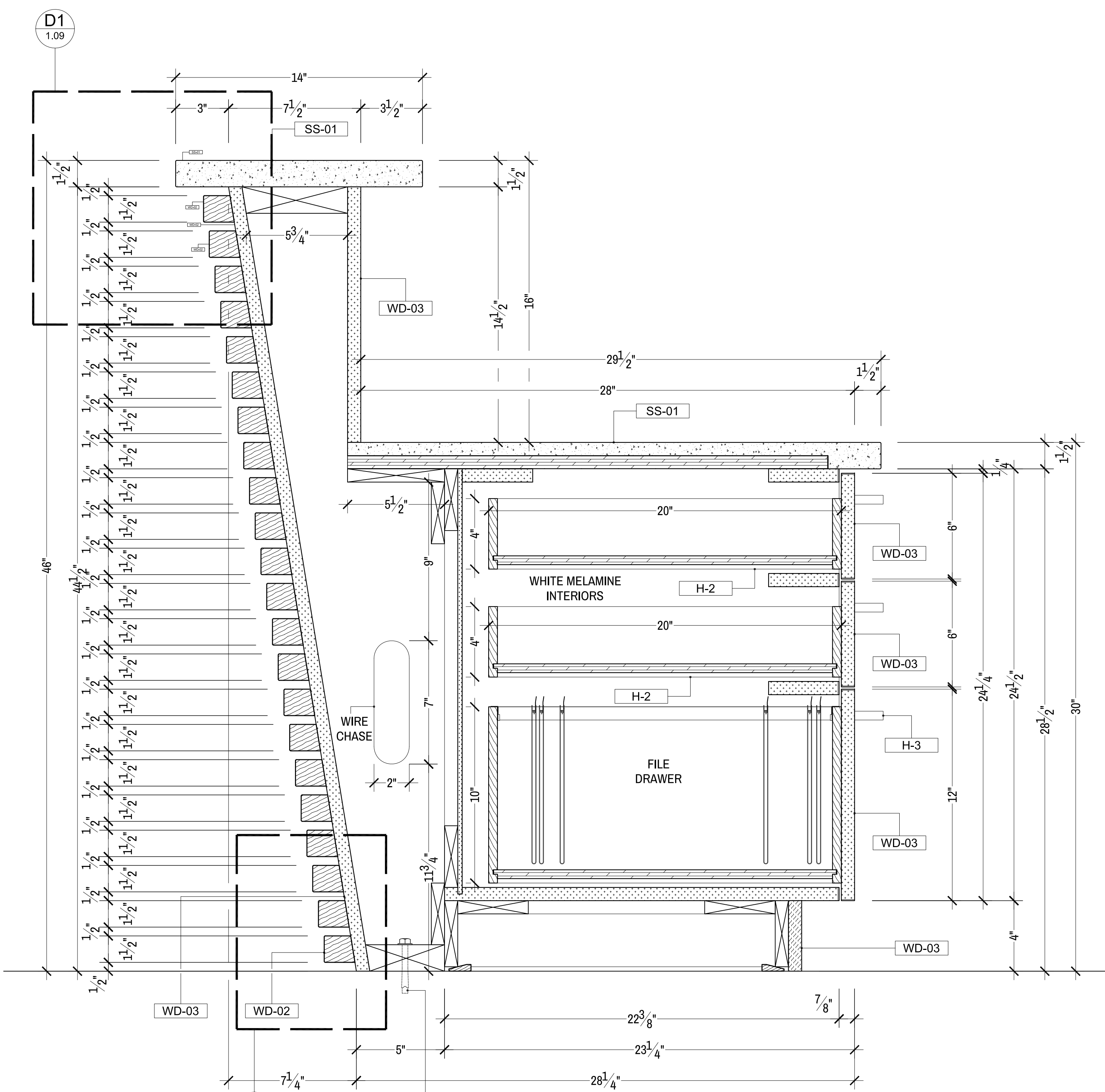
S2 SECTION SCALE: 3"=1'-0" RECEPTION RECEPTION 105
